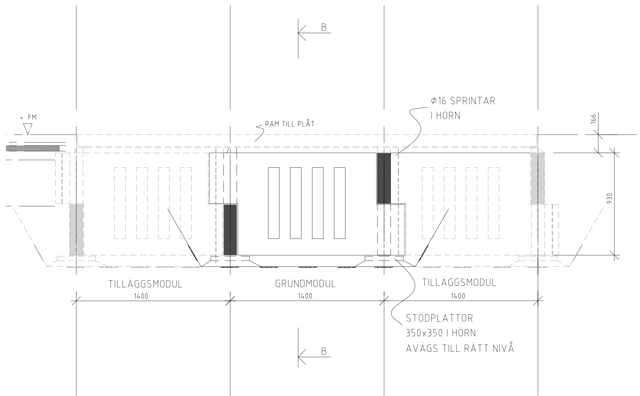
A 1:20 ELEVATION
